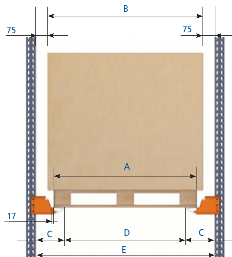
Figure 2. The load overhangs the pallet
